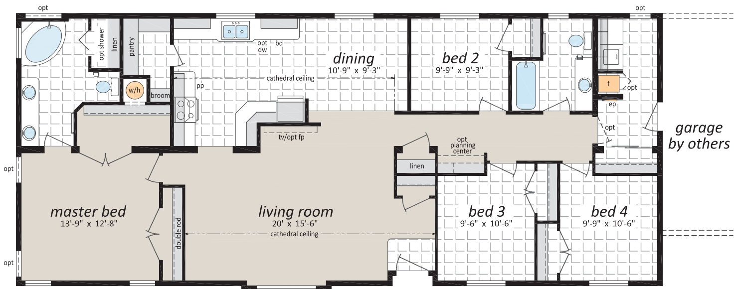
The Norfolk ST-7641 27' x 64' • 1,728 sq. ft.
