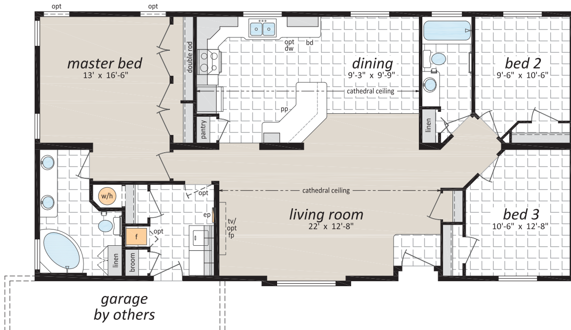
The Cornwall ST-7542 27' x 54' • 1,458 sq. ft.
