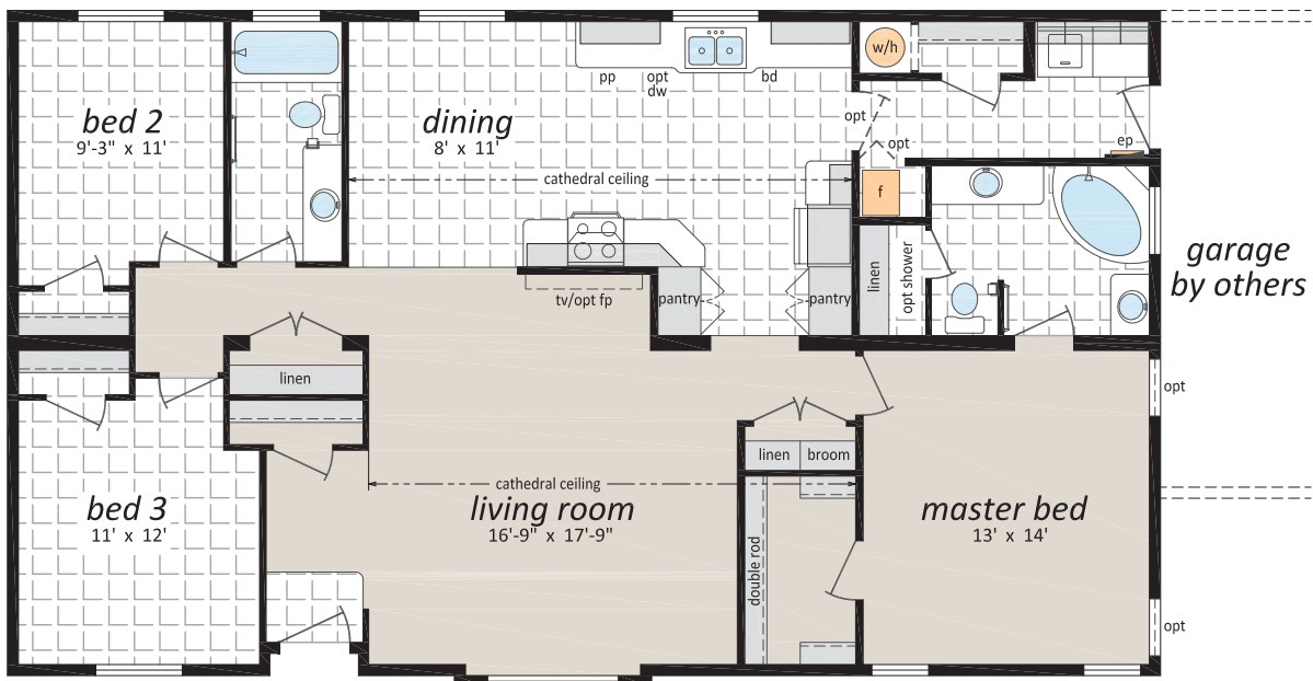
The Suffolk ST-3521 30' x 52' • 1,560 sq. ft.
