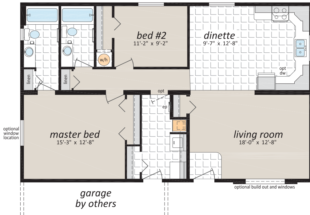
"The Montrose" CDF-244 27' x 44' 1,188 sq. ft.
