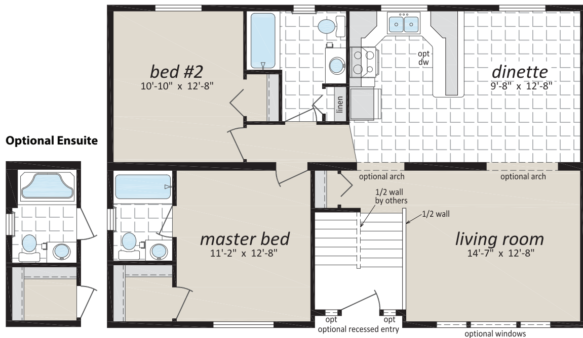
"The Wenatchee" CDF-230 27' x 40' 1,080 sq. ft.
