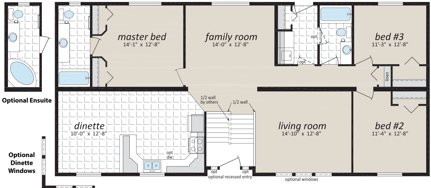
"The Mackenzie" CDF-215 27' x 58' 1,566 sq. ft.
