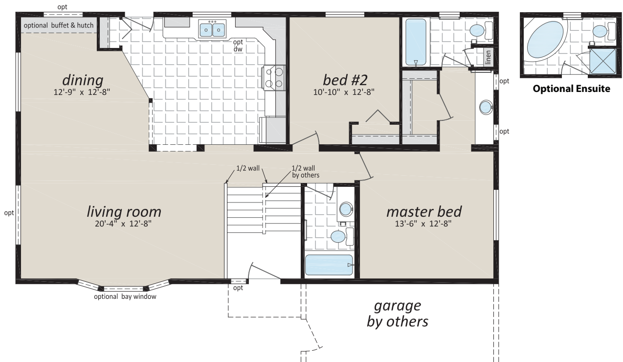
"The Chemainus" CDF-201 27' x 48' 1,296 sq. ft.
